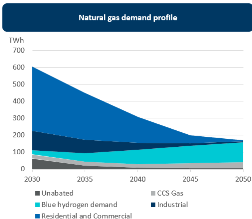
Figure 4-7: Demand profile for natural gas (TWh), 2030-2050
