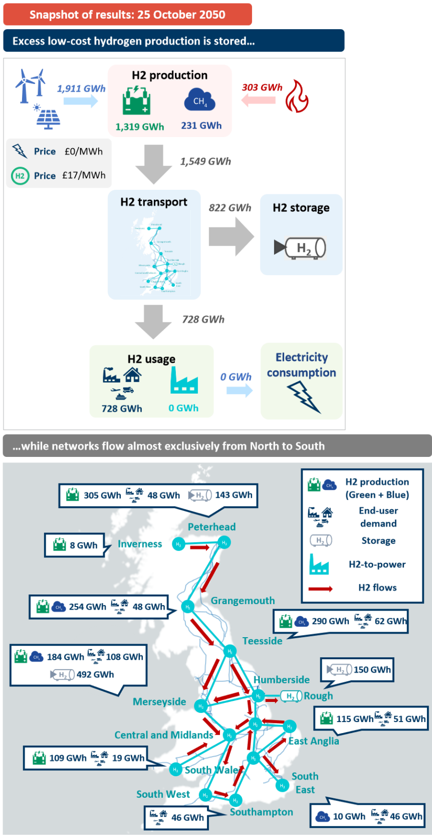
Figure 8-1: Hydrogen flows on a windy day in 2050
