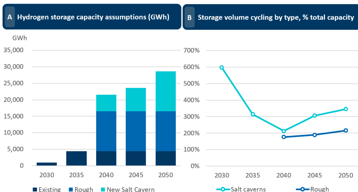
Figure 8-5: A) Hydrogen storage capacity (GWh) and B) cycling rates (%) in our modelled scenario, 2030 to 2050
