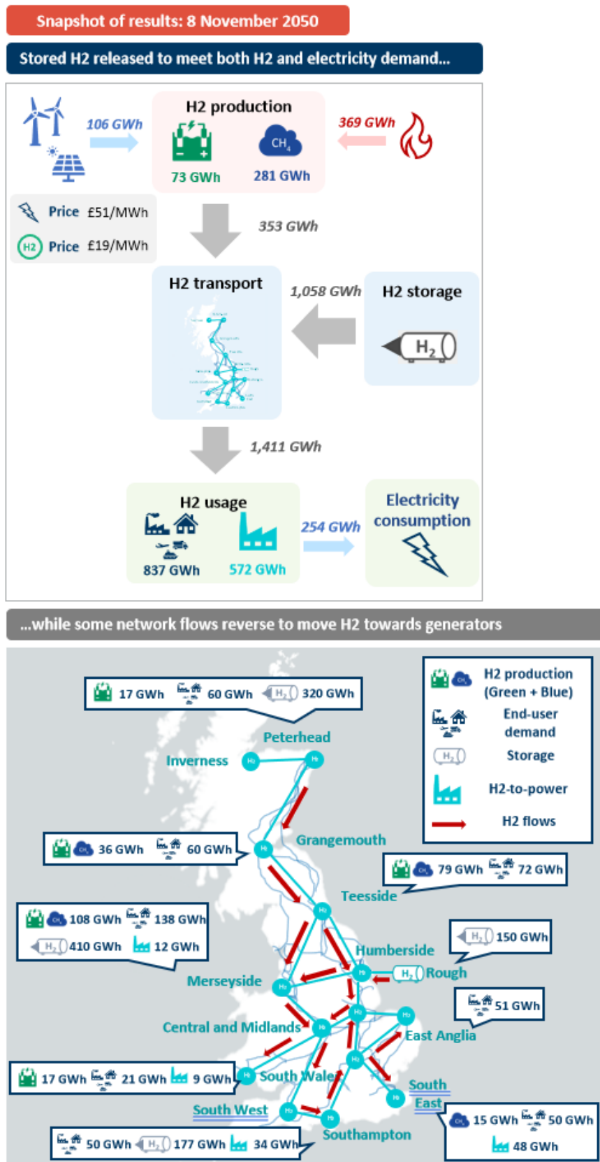
Figure 8-2: Hydrogen flows on a low-wind day in 2050
